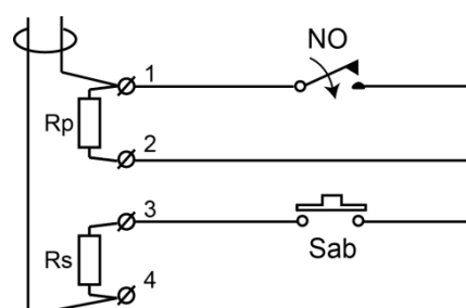
Fig. 4. MC 440-PRpSRs with build in resistors:
