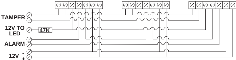
Figure 2: Multiple Unit Connection Procedure
