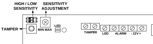
Figure 1: Terminal Connections Diagram
