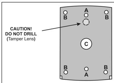
Figure 1: Back Plate
