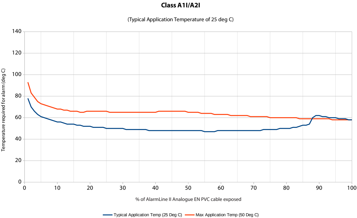
Chart 1 - Expected temperature required for an alarm in relation to percentage of AlarmLine II Analogue EN LHD Cable in Class A1I/A2I Setting
