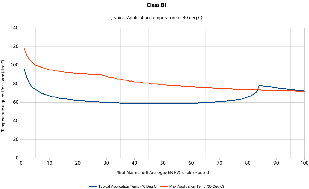
Chart 2 - Expected temperature required for an alarm in relation to percentage of AlarmLine II Analogue EN LHD Cable in Class BI Setting
