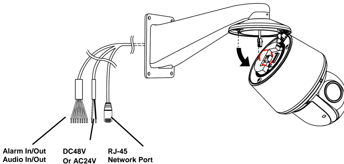
FIGURE 2-6: CONNECTING THE WIRES
