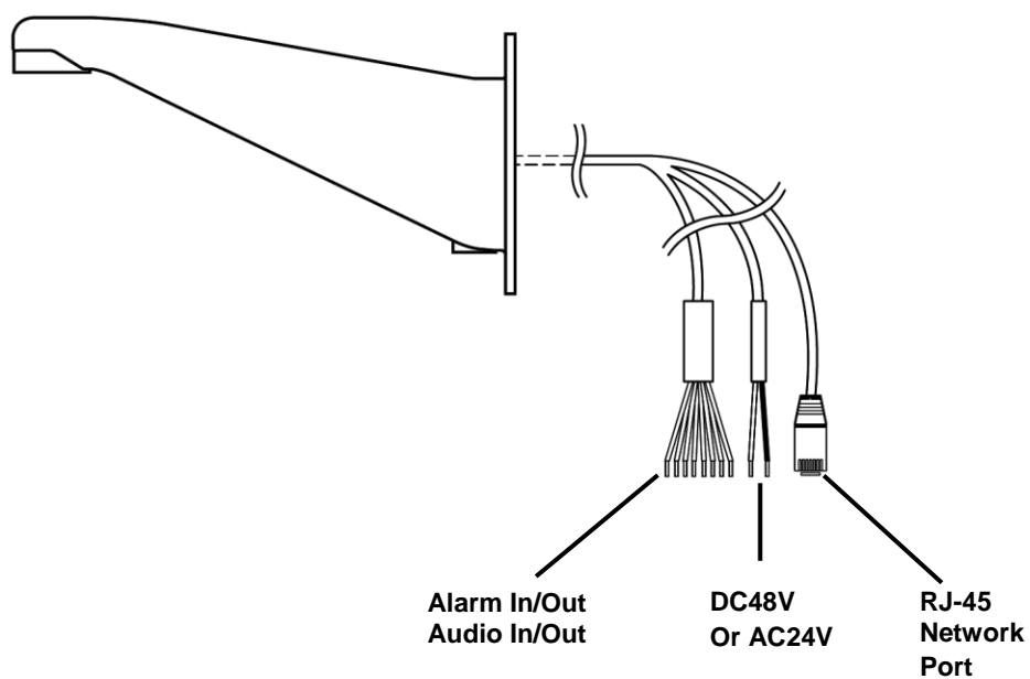
FIGURE 2-2: ROUTING THE CABLES
