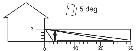
Figure 2: Sensor 3m high, 5 degree tilt, 30m range
