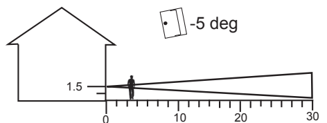
Figure 4: Sensor 1.5m high, -5 degree tilt, 30m range
