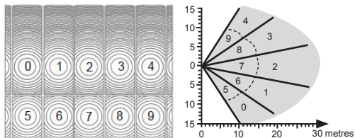
Figure 4: Sensor 1.5m high, -5 degree tilt, 30m range
