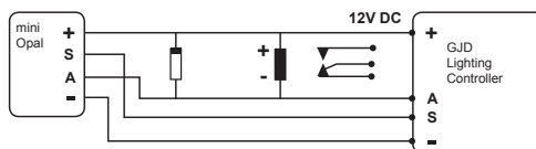
Figure 8: External relay wiring diagram
