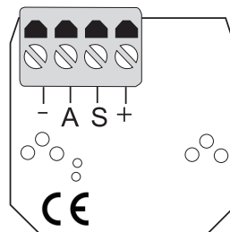
Figure 6: Rear of PCB with Connections
