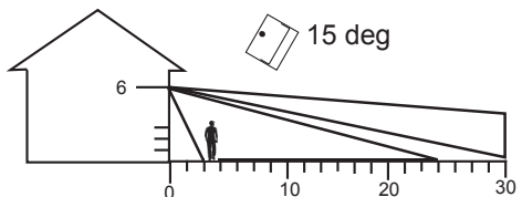
Figure 3: Sensor 6m high, 15 degree tilt, 30m range
