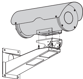
Fig. 6 Bracket mounting.
