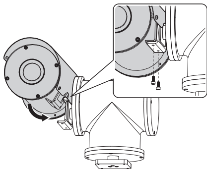
Fig. 7 P&T installation.
