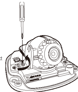
Fixing Hole
