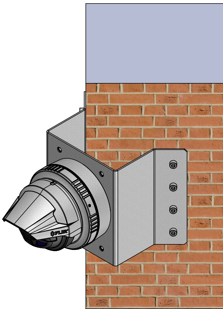
CORNER MOUNT ASSY- GEN-X SERIES PN (421-0066-00) SHEET 4
