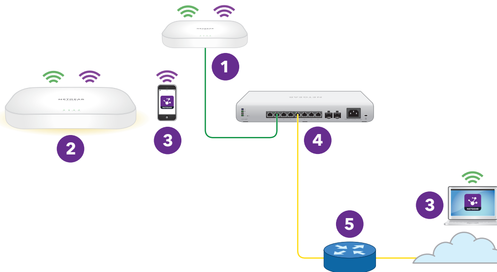
Figure 5. Mesh network with an extender access point and a wired root access point
