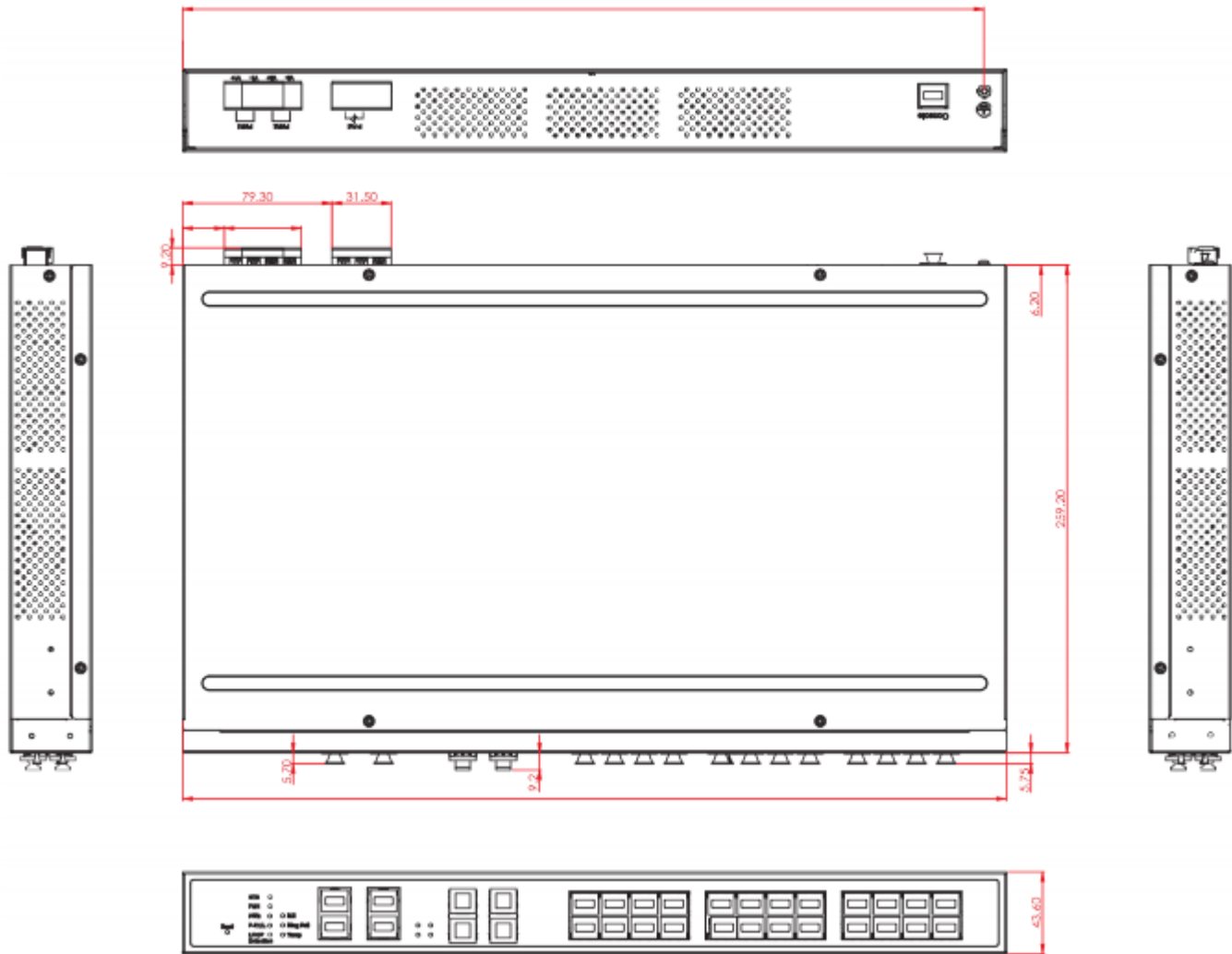
Figure 1-4. CNGE28FX4TX24MSPOE2/48 Dimensions
