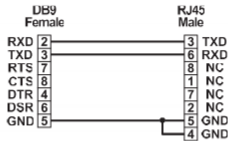
Figure 2-11. Pin Assignment
