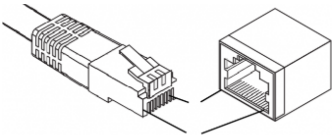
Figure 2-8. Ethernet Plug & Connector Pin Position
